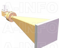
LB-15-25-C-1.85FSPO Standard Gain Horn Antenna 50-65GHz 25dB Gain 1.85mm Female
