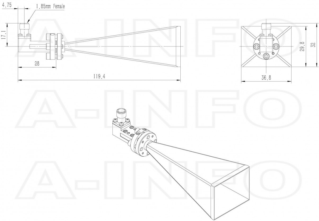
1.85mm-Female Output (P/N: LB-15-25-C-1.85F)
